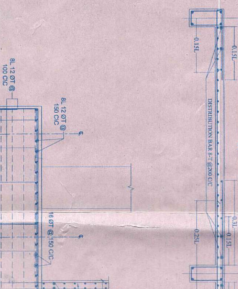
TYPICAL SECTION OF SLAB
