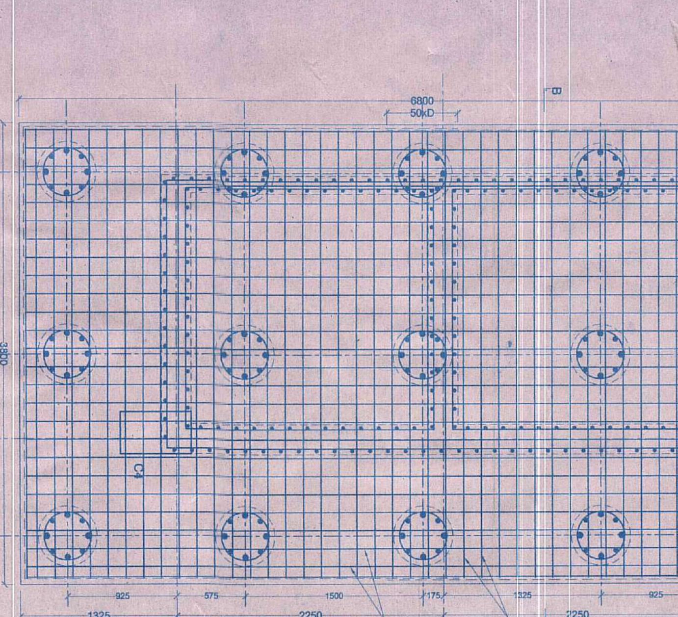
PLAN
