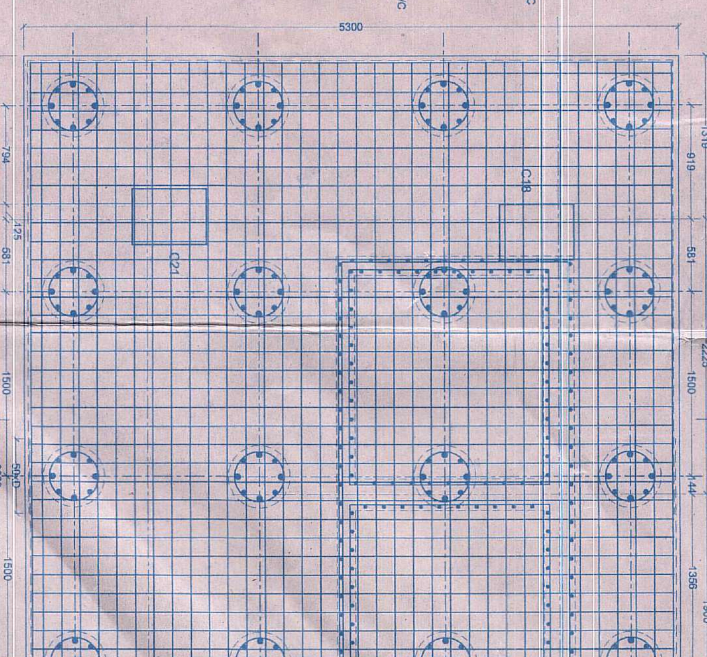
SECTION A1-B-B
